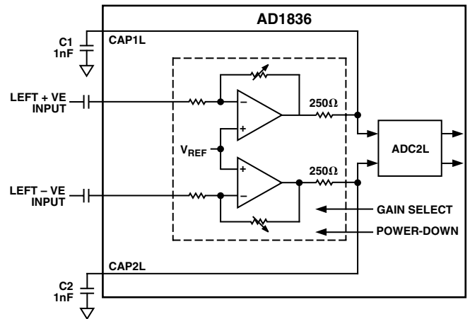
Figure 13. Differential Mode
