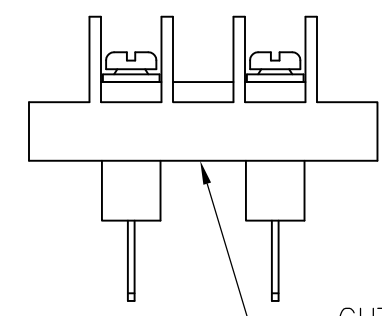
2-796985-3 CUT TURRET OFF FLUSH WITH BOTTOM OF HOUSING
