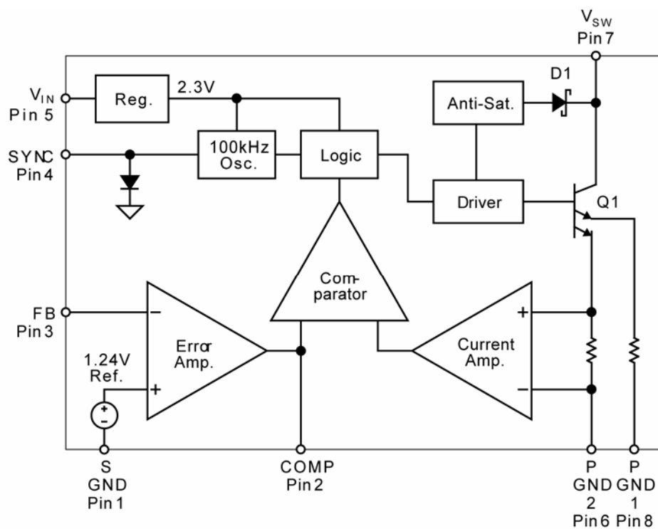
MIC2172 Block Diagram
