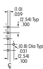
AB11 model does not have terminal 2. AB15AV-FA
