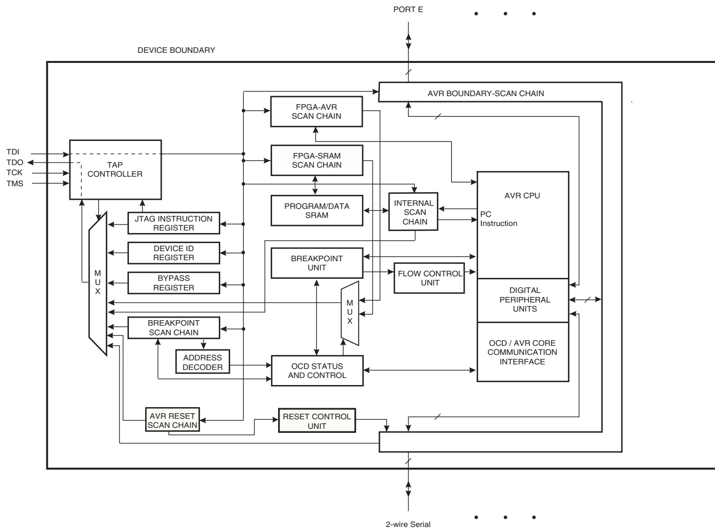
Figure 39. Block Diagram
