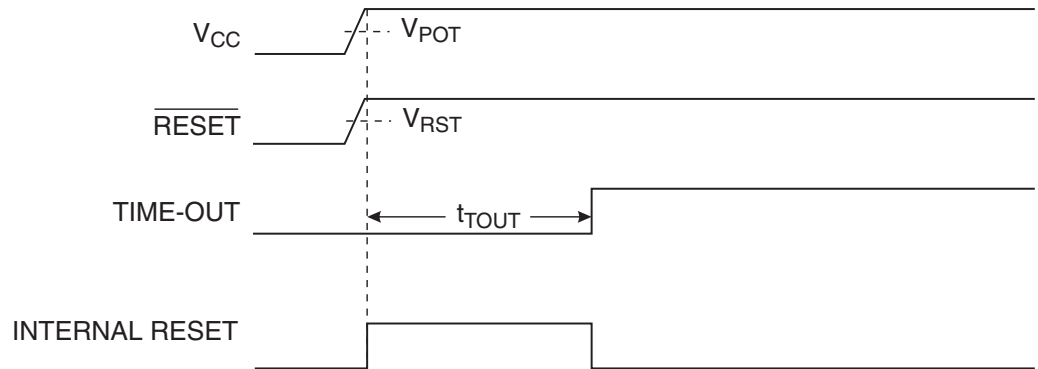
Figure 36. MCU Start-up, RESET Tied to V_{CC}
