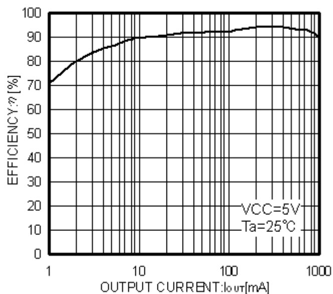
Figure 15. Efficiency
