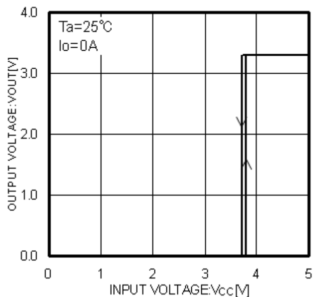
Figure 11. V_{OUT} VS V_{CC}
