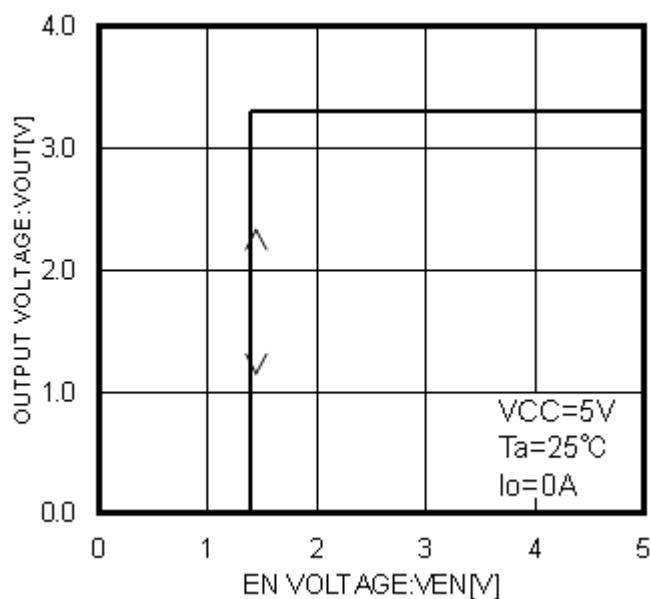
Figure 12. V_{OUT} VS V_{EN}
