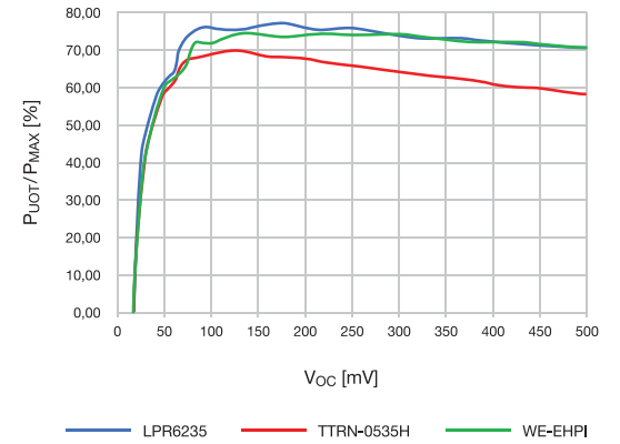
Efficiency vs V_{OC} for MCRY12-125Q-42*I with R_{TEG}=12\Omega and V_{OUT}=3.0\text{V}
