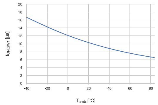
LX1-switch on-time vs T_{amb} for MCRY12-125Q-42*I
