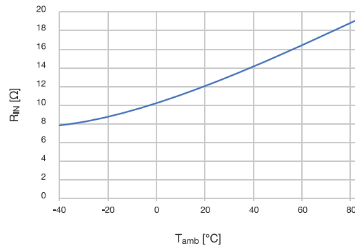
R_{IN} (calculated from t_{ON,SW1} and f ) vs T_{amb} for MCRY12-125Q-42*I and L_1=12.5\mu\text{H}
