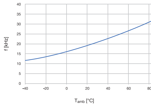
Switching Frequency vs T_{amb} for MCRY12-125Q-42*I
