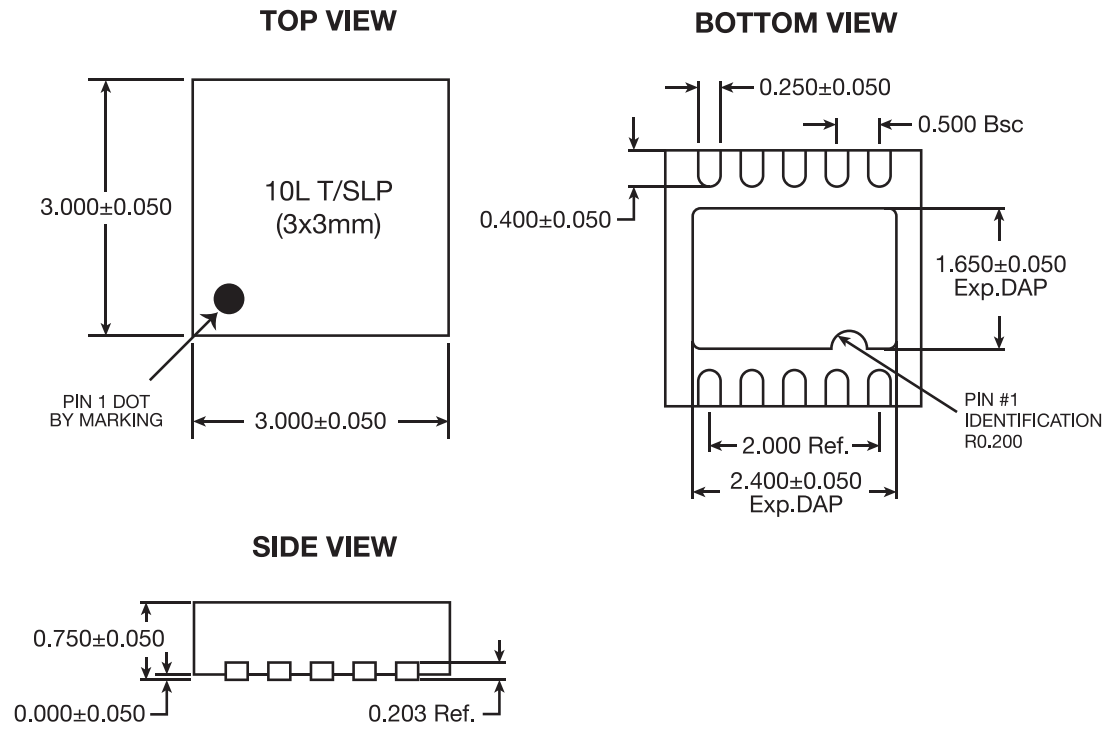
Figure 8: Package drawing of 10-lead, 3mm × 3mm DFN
