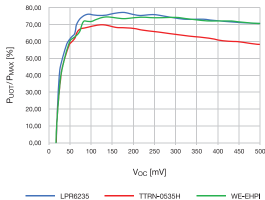
Efficiency vs V_{OC} for MCRY12-125Q-42*I with R_{TEG}=12\Omega and V_{OUT}=3.0\text{V}
