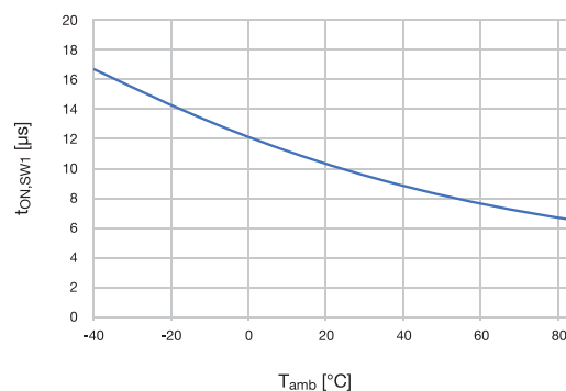
LX1-switch on-time vs T_{amb} for MCRY12-125Q-42*I
