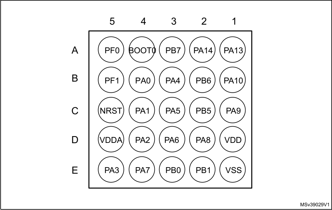
Figure 7. WLCSP25 25-ball package ballout (bump side)
