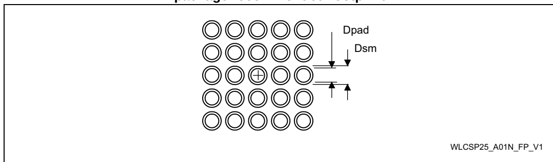
Figure 44. WLCSP25 - 25-ball, 2.133 x 2.070 mm, 0.4 mm pitch wafer level chip scale package recommended footprint
