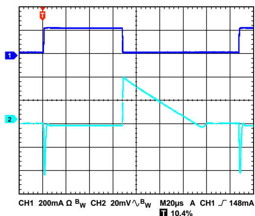
Figure 38. Load Transient Response, I_{LOAD} = 1\text{ mA} to 200\text{ mA} , V_{OUT} = 3.3\text{ V} , V_{IN} = 5\text{ V} , CH1 Load Current, CH2 V_{OUT}
