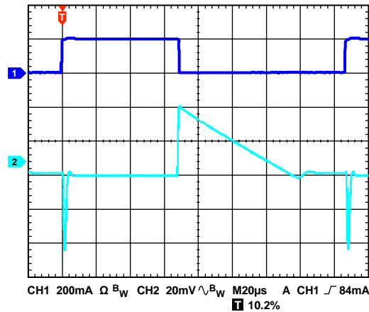
Figure 40. Load Transient Response, I_{LOAD} = 1\text{ mA} to 200\text{ mA} , V_{OUT} = 1.8\text{ V} , V_{IN} = 3\text{ V} , CH1 Load Current, CH2 V_{OUT}
