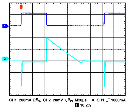
Figure 36. Load Transient Response, I_{LOAD} = 1\text{ mA} to 200\text{ mA} , V_{OUT} = 5\text{ V} , V_{IN} = 7\text{ V} , CH1 Load Current, CH2 V_{OUT}
