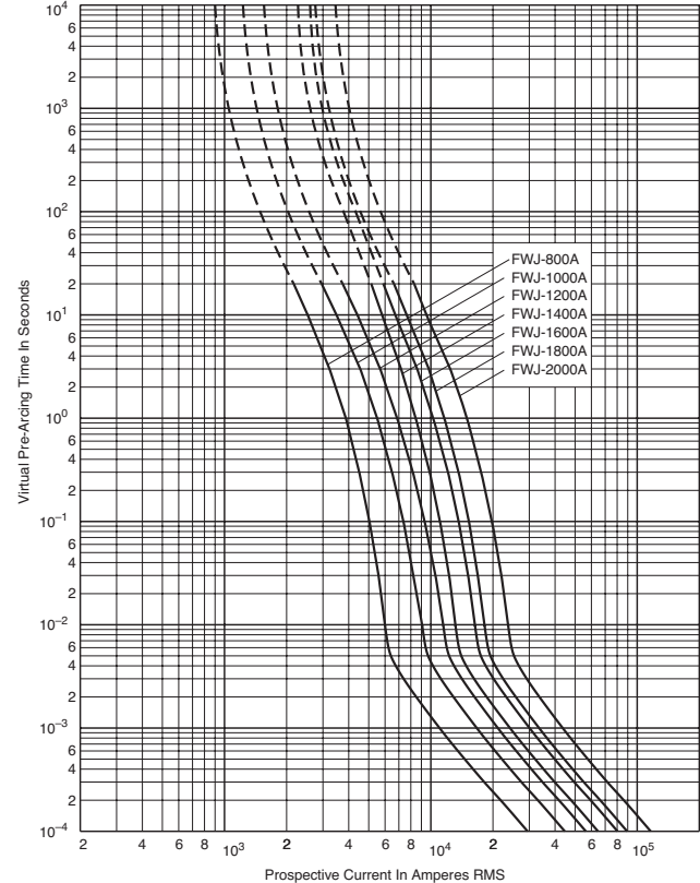
Time-Current Curve
