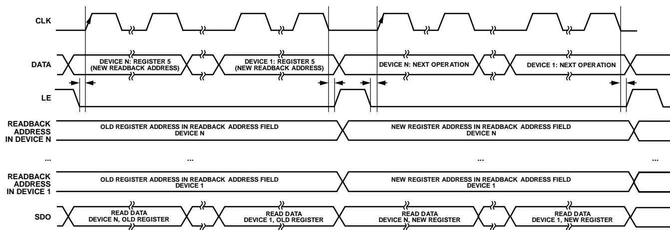
Figure 49. Timing Diagram for Readback from Multiple Devices Using Daisy-Chain Functionality for N Devices
