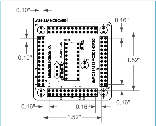
Figure 30: Dimensions of MCU card for MCU Card 10
