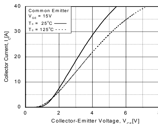
Figure 2. Typical Saturation Voltage Characteristics
