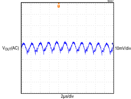
MAXM15466 OUTPUT VOLTAGE RIPPLE V_{IN} = 24V , FIXED V_{OUT} = 5V FULL LOAD, PWM MODE
