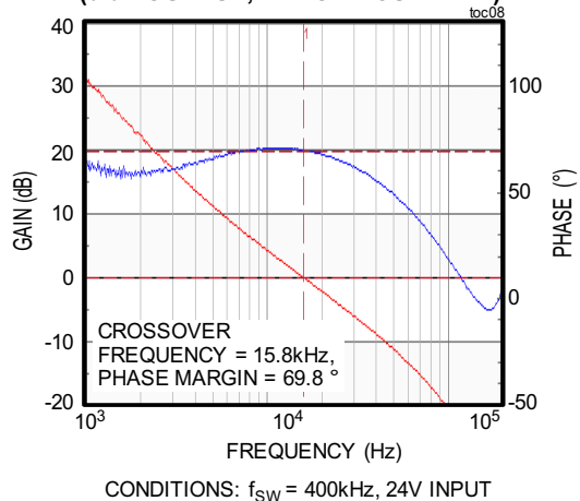
BODE PLOT (3.3V OUTPUT, 1A LOAD CURRENT)
