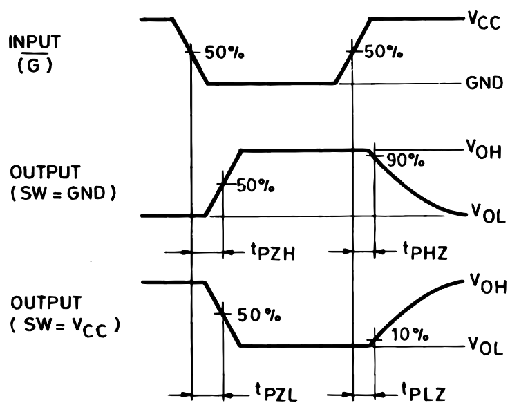
Figure 5: Output Enable And Disable Times Waveform ( f=1\text{MHz} ; 50% duty cycle)
