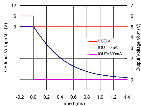
R1518x50xF ( C_2 = 0.1 \mu\text{F} , C_D = 1 \text{ nF} )
