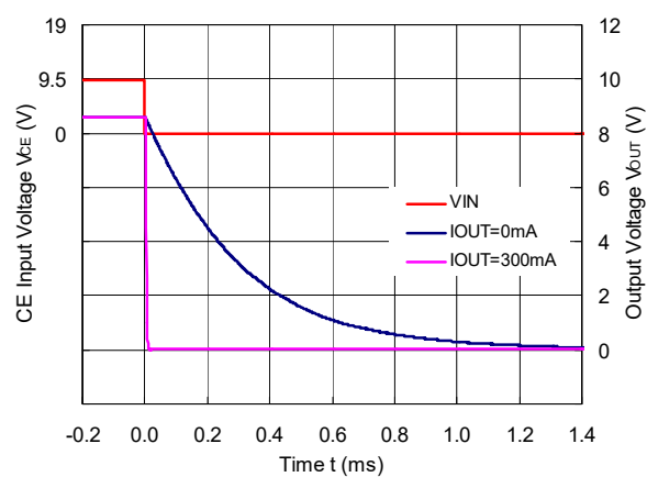
R1518x85xF ( C_2 = 0.1 \mu\text{F} , C_D = 1 \text{ nF} )
