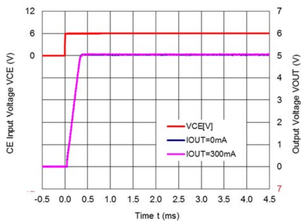
R1518J851E/F ( C_2 = 0.1 \mu\text{F} , C_D = 1 \text{ nF} )
