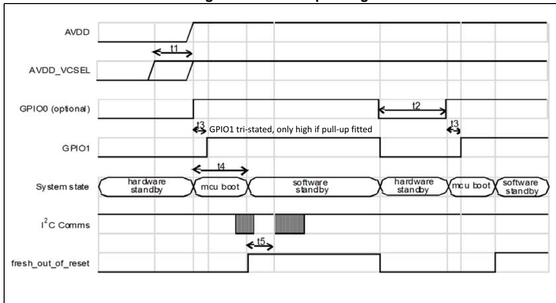
Figure 10. Power-up timing
