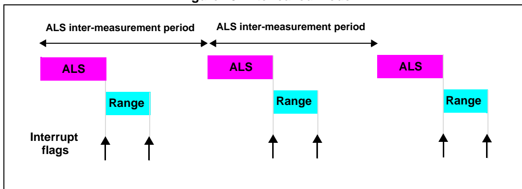
Figure 19. Interleaved mode
