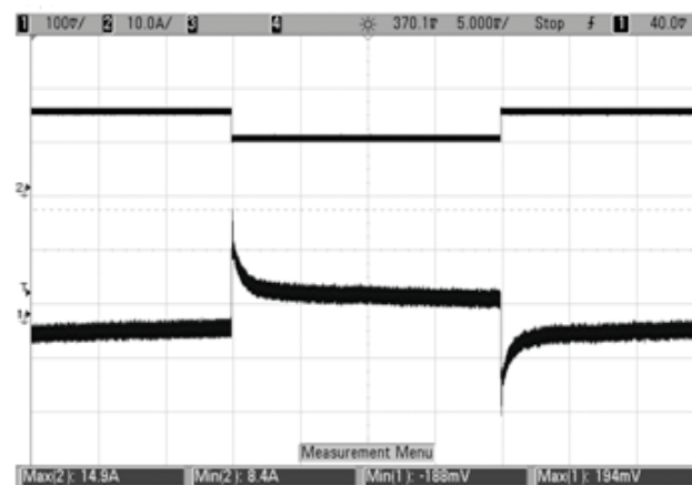
Stepload Transient Response (Vin = 48V, Cload = 470uF, Iout = 50-75-50% of Imax, 1A/μS, Ta = +25°C)
