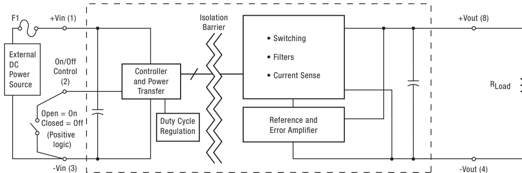
Figure 1. Connection Diagram
