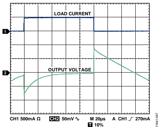
Figure 63. Output Transient Response, V_{OUT} = 1.8\text{ V} , C_{OUT} = 1\text{ }\mu\text{F}
