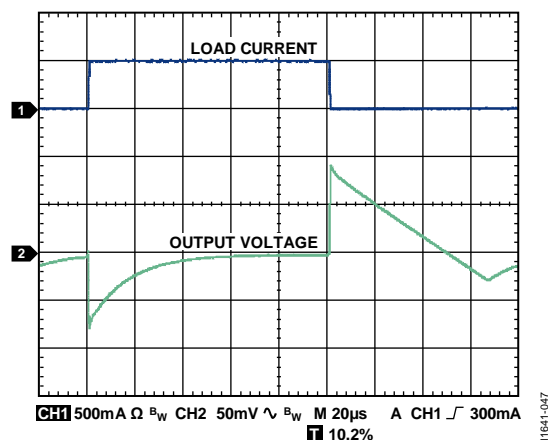
Figure 53. Load Transient Response, C_{IN} = C_{OUT} = 1 \mu F , I_{LOAD} = 1 \text{ mA} to 500 mA, V_{OUT} = 5 \text{ V} , V_{IN} = 7 \text{ V}
