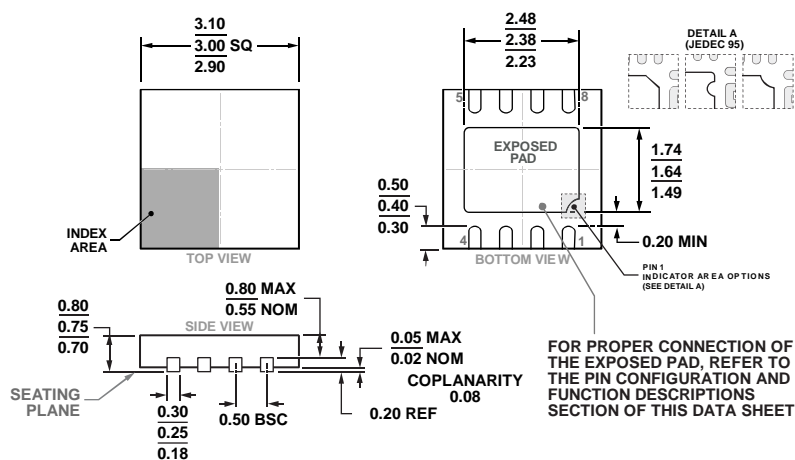
Figure 81. 8-Lead Lead Frame Chip Scale Package [LFCSP]
