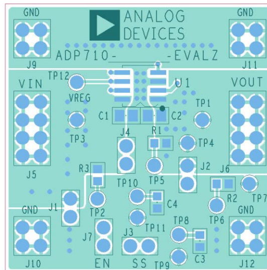
Figure 80. Example SOIC PCB Layout
