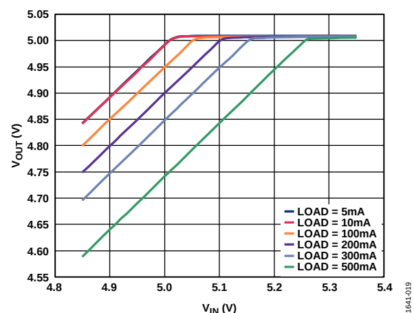
Figure 21. Output Voltage vs. Input Voltage (in Dropout), V_{OUT} = 5\text{ V}
