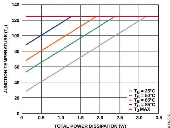
Figure 78. SOIC
