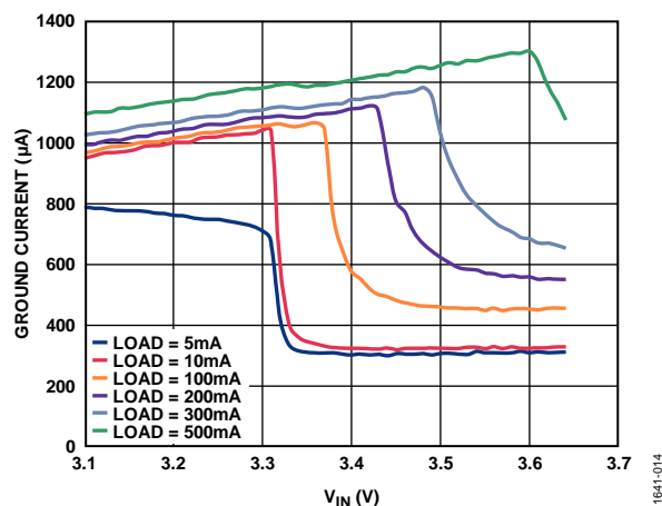
Figure 14. Ground Current vs. Input Voltage (in Dropout), V_{OUT} = 3.3 V
