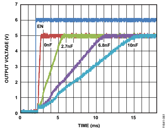
Figure 67. Typical Start-Up Behavior
