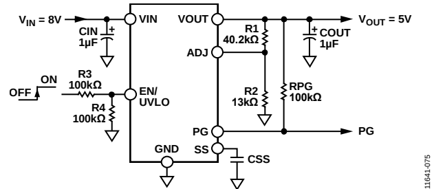
Figure 62. Typical Adjustable Output Voltage Application Schematic
