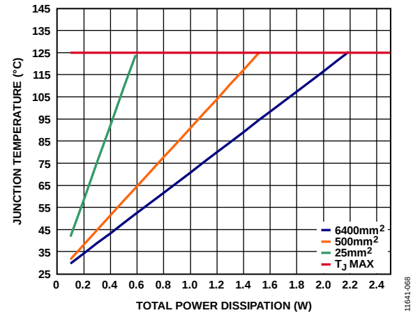
Figure 74. SOIC, T_A = 25^{\circ}\text{C}
