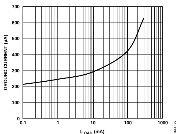
Figure 27. Ground Current vs. Load Current, V_{OUT} = 1.8\text{ V}
