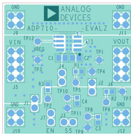
Figure 80. Example SOIC PCB Layout
