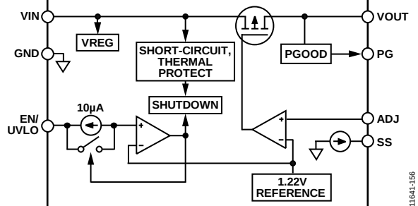
Figure 61. Adjustable Output Voltage Internal Block Diagram
