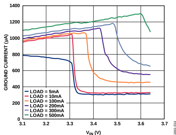
Figure 14. Ground Current vs. Input Voltage (in Dropout), V_{OUT} = 3.3\text{ V}
