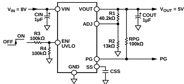
Figure 62. Typical Adjustable Output Voltage Application Schematic
