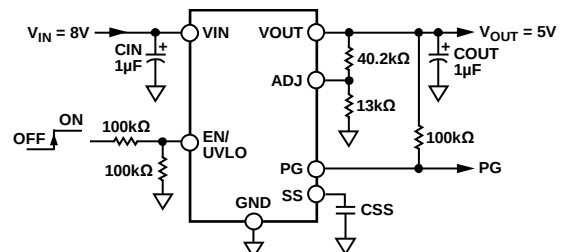
Figure 2. ADP7105 with Adjustable Output Voltage, 5 V
