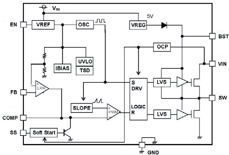
Figure 3. Block Diagram
