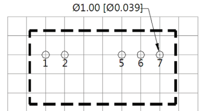
Top View PCB LAYOUT
