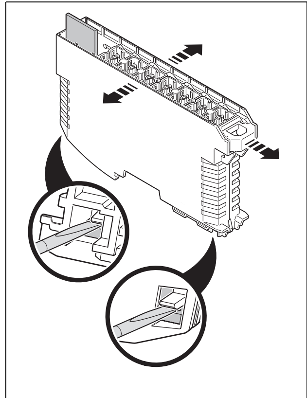
Figure 45 Taking out the PCB
