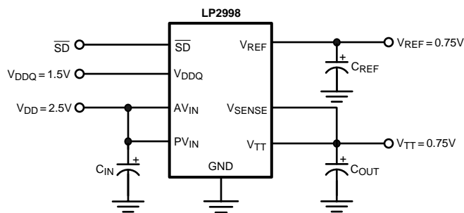
Figure 30. HSTL Application
