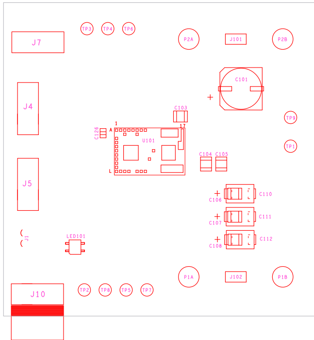
FIGURE 3. ASSEMBLY TOP
