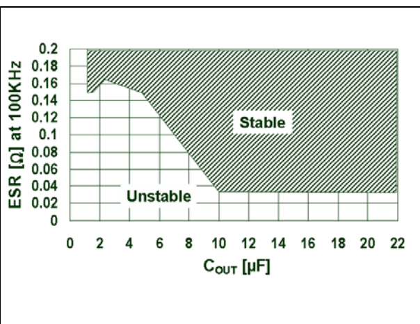
Figure 18. Stable region vs. C_{OUT} and low ESR
