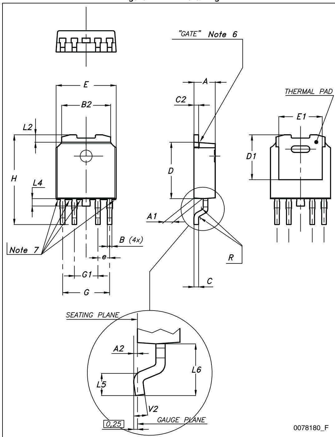
Figure 24. PPAK drawing
