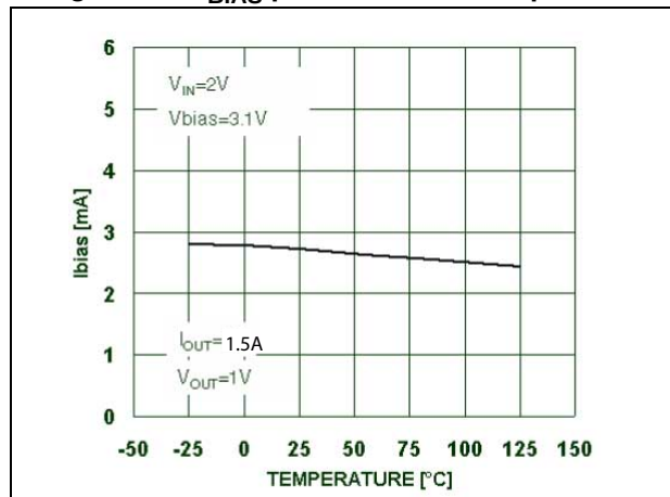
Figure 13. V_{BIAS} pin current vs. temperature
