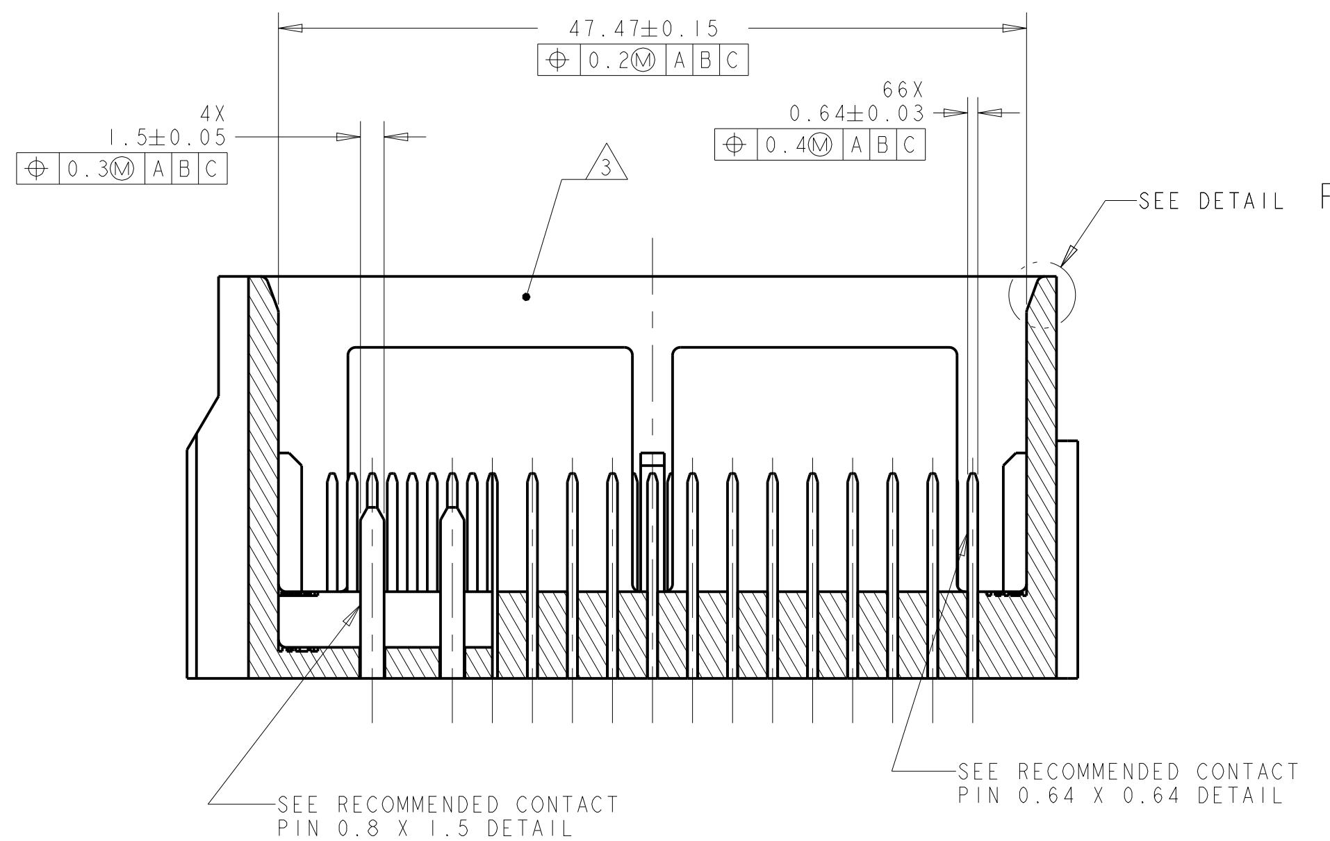
SECTION B-B
