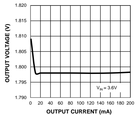
Output Voltage vs. Output Current (DCM)
