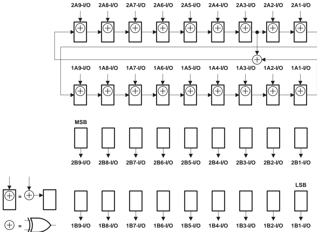
Figure 12. 18-Bit PSA/COUNT Configuration (1OEAB = 2OEAB = 1, \overline{1OEBA} = \overline{2OEBA} = 1 )
