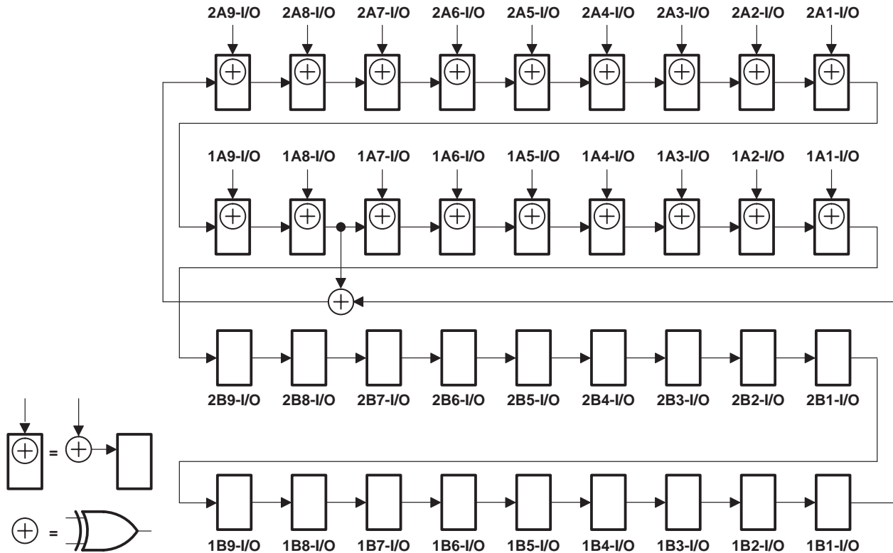
Figure 8. 36-Bit PSA Configuration (1OEAB = 2OEAB = 1, \overline{1OEBA} = \overline{2OEBA} = 1 )
