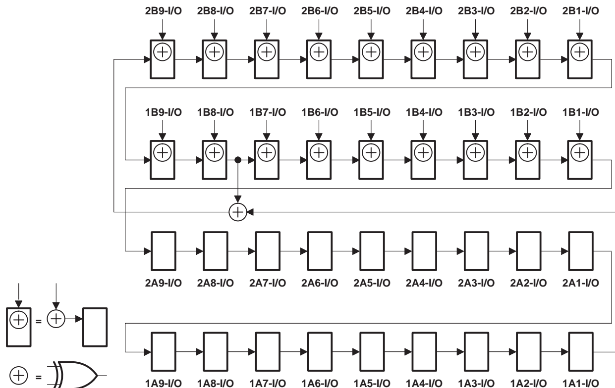
Figure 9. 36-Bit PSA Configuration ( 1OEAB = 2OEAB = 0 , 1\overline{OEBA} = 2\overline{OEBA} = 0 )
