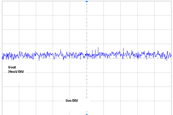
FIGURE 10. OUTPUT RIPPLE
