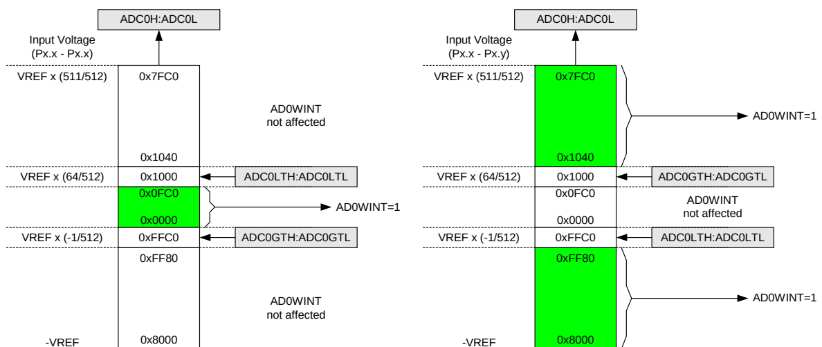
Figure 5.9. ADC Window Compare Example: Left-Justified Differential Data
