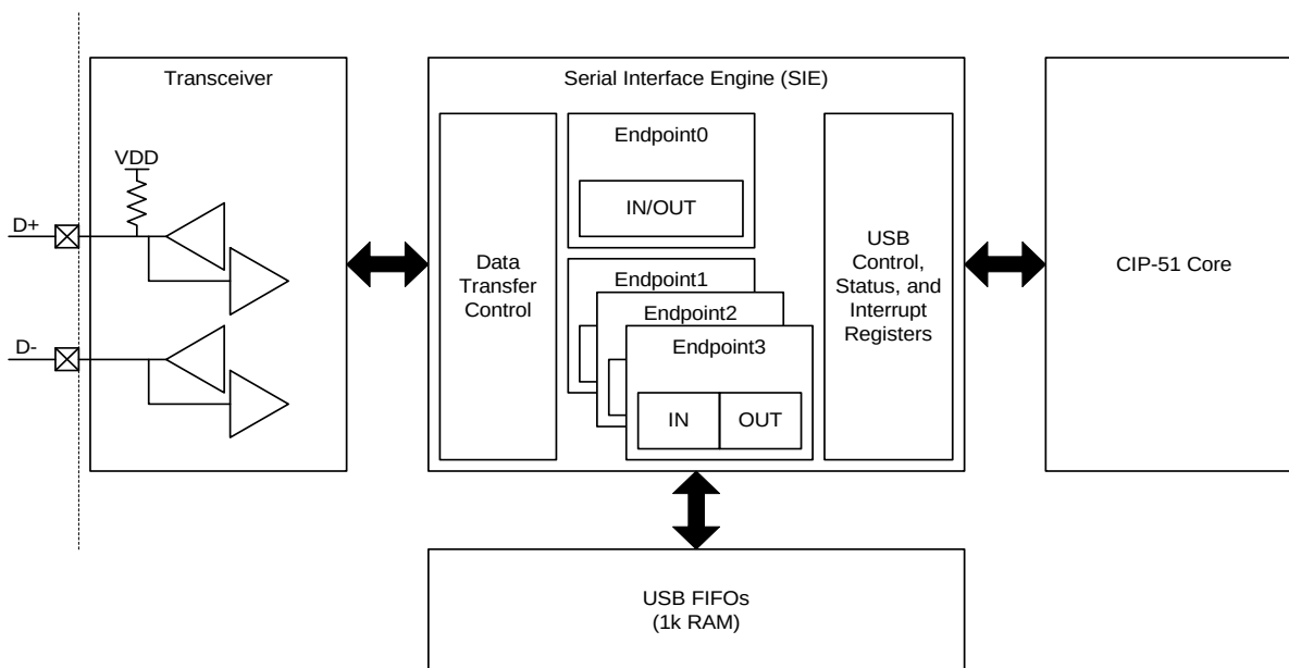
Figure 16.1. USB0 Block Diagram
