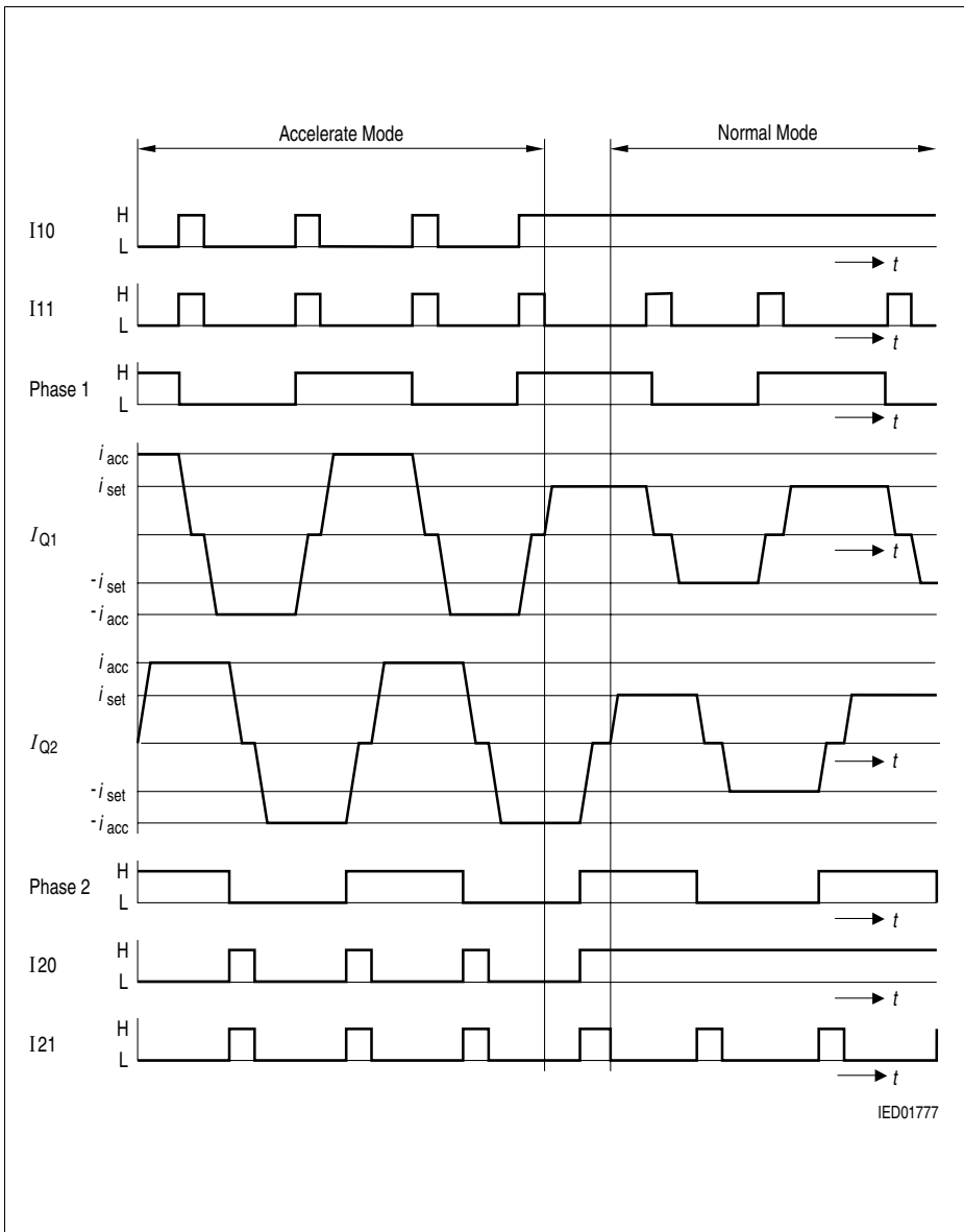
Figure 6 Half-Step Operation
