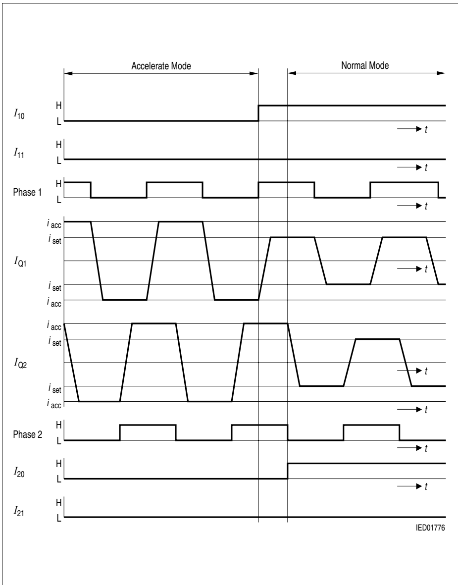
Figure 5 Full-Step Operation
