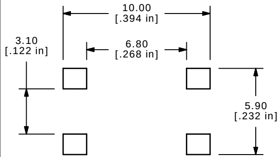
P.C.B MOUNTING
