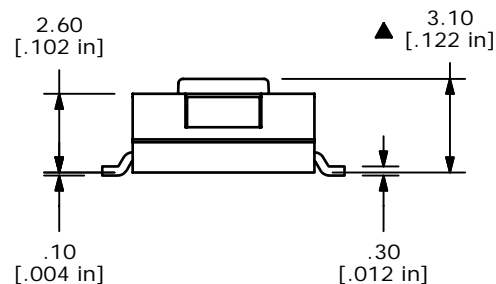
TERMINALS TO BE COLPLANAR WITH IN 0.10mm
