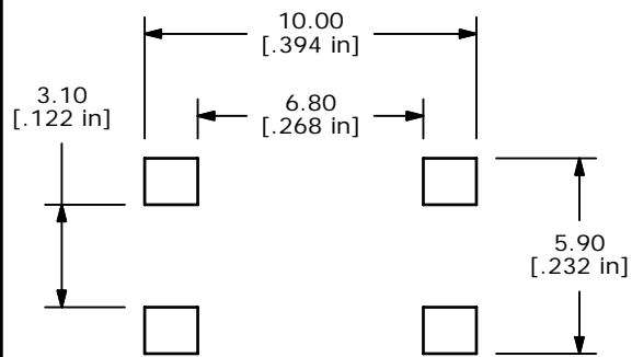
P.C.B MOUNTING
