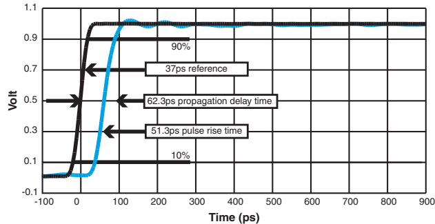
SRF300/SRF303 Time Response (RF Note 6)
