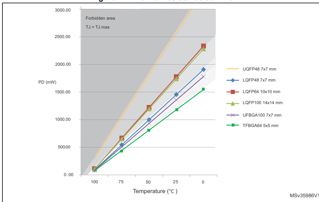
Figure 47. Thermal resistance suffix 6
