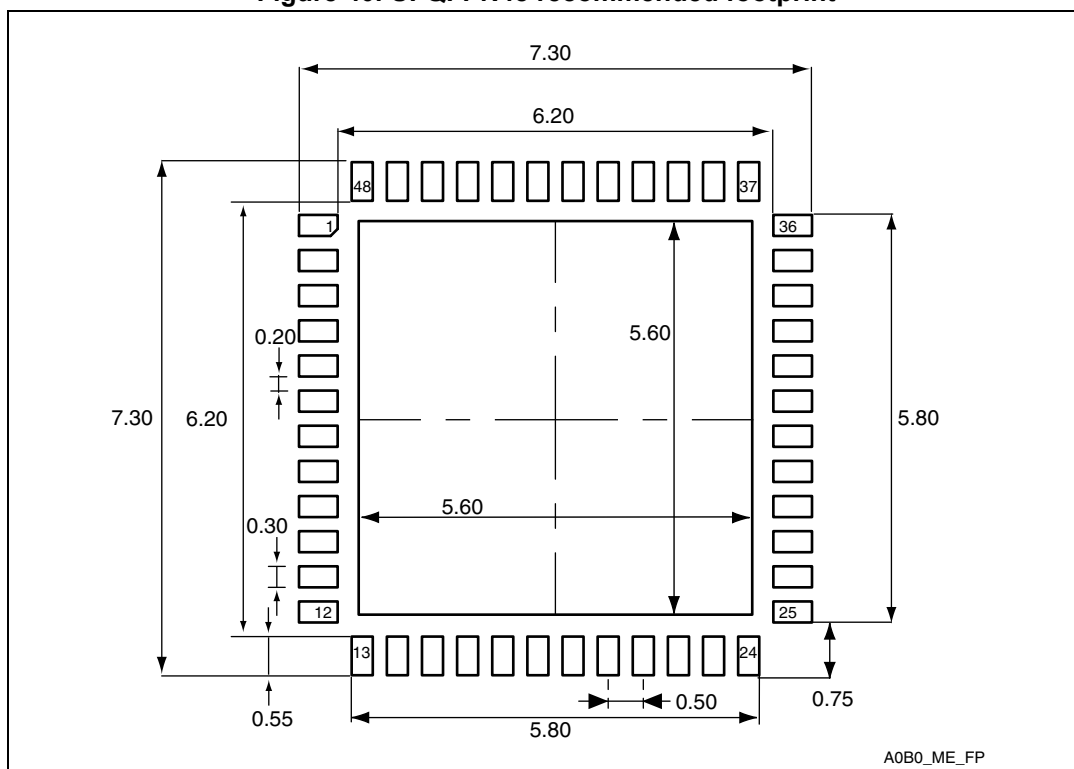
Figure 40. UFQFPN48 recommended footprint
