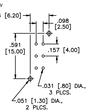
P.C. BOARD LAYOUT
