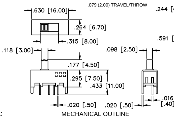
MECHANICAL OUTLINE
