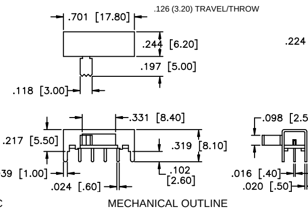
MECHANICAL OUTLINE
