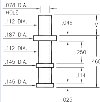
2817-X-00-XX-00-00-07-0 Swage mount in .116 hole
