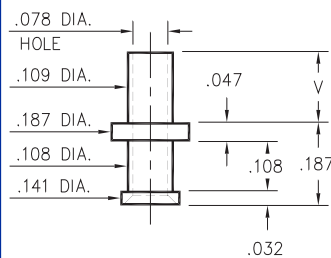
2815-X-00-XX-00-00-07-0 Swage mount in .113 hole
