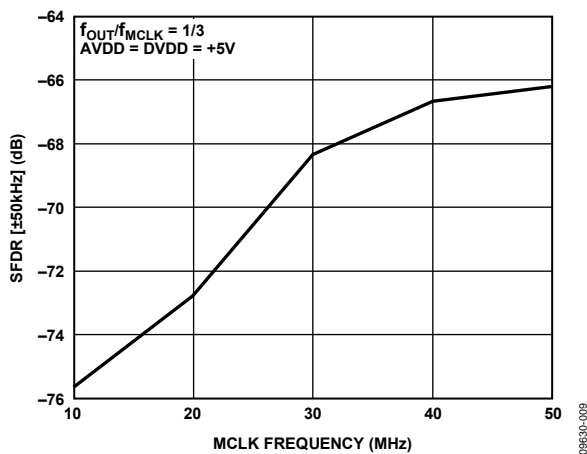
Figure 9. Narrow-Band SFDR vs. MCLK Frequency
