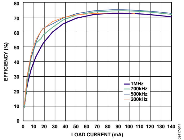
Figure 14. 5 V In to 15 V Out Efficiency with the Halo Transformer at Various Switching Frequencies
