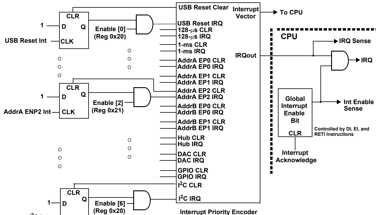
Figure 16-3. Interrupt Controller Function Diagram
